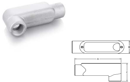
LL Form 5 Material:Malleable Iron Finish:Zinc Plated+Alum Painting
