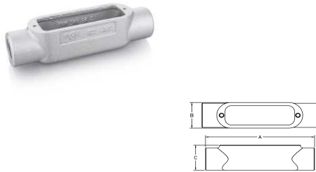
C Form 8 Material:Grey Iron Finish:Zinc Plated+Alum Painting
