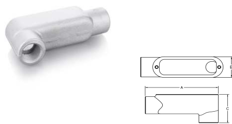
LB Form 8 Material:Grey Iron Finish:Zinc Plated+Alum Painting
