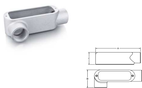
LR Form 8 Material:Grey Iron Finish:Zinc Plated+Alum Painting
