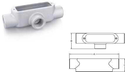
T Form 5 Material:Malleable Iron Finish:Zinc Plated+Alum Painting
