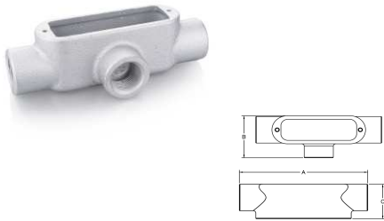
T Form 8 Material: Grey Iron Finish: Zinc Plated+ Alum Painting
