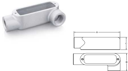
LL Form 5 Material:Malleable Iron Finish:Zinc Plated+Alum Painting
