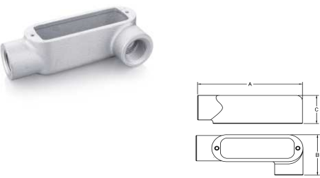
LL Form 8 Material:Grey Iron Finish:Zinc Plated+Alum Painting
