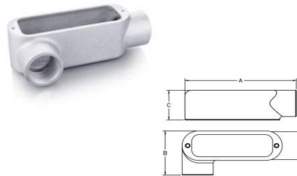
LR Form 5 Material:Malleable Iron Finish:Zinc Plated+Alum Painting
