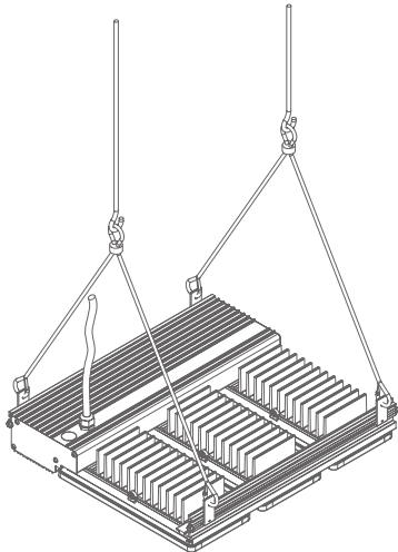
Aircraft cable • Ships separately from fixture • For mounting with or without dust cover
