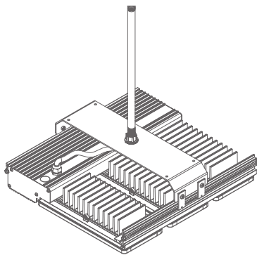
Pendant mount • P1 and P2 for use without dust cover; can be ordered separately or factory installed • P3 and P4 for use with dust cover
